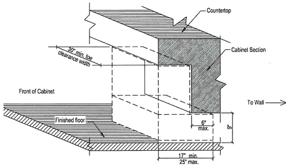
Figure 1 - Toe Clearance
