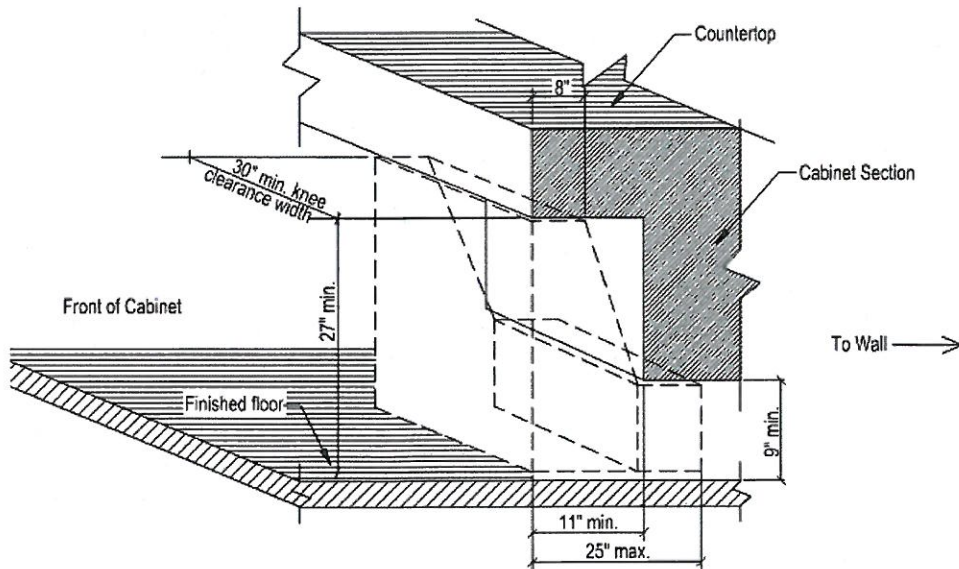
Figure 2 - Knee Clearance
